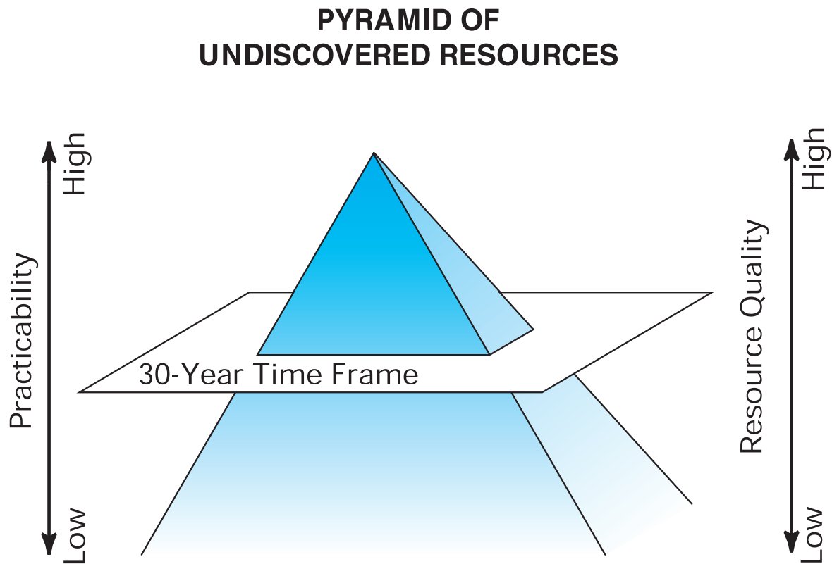
Figure 1. Sketch depicting a 30-year resource-assessment forecast span as a slice through the conventional-accumulation resource pyramid at some quality level. Accumulation categories below the selected slice level are excluded from assessment consideration. (Modified from McCabe, 1998.)
