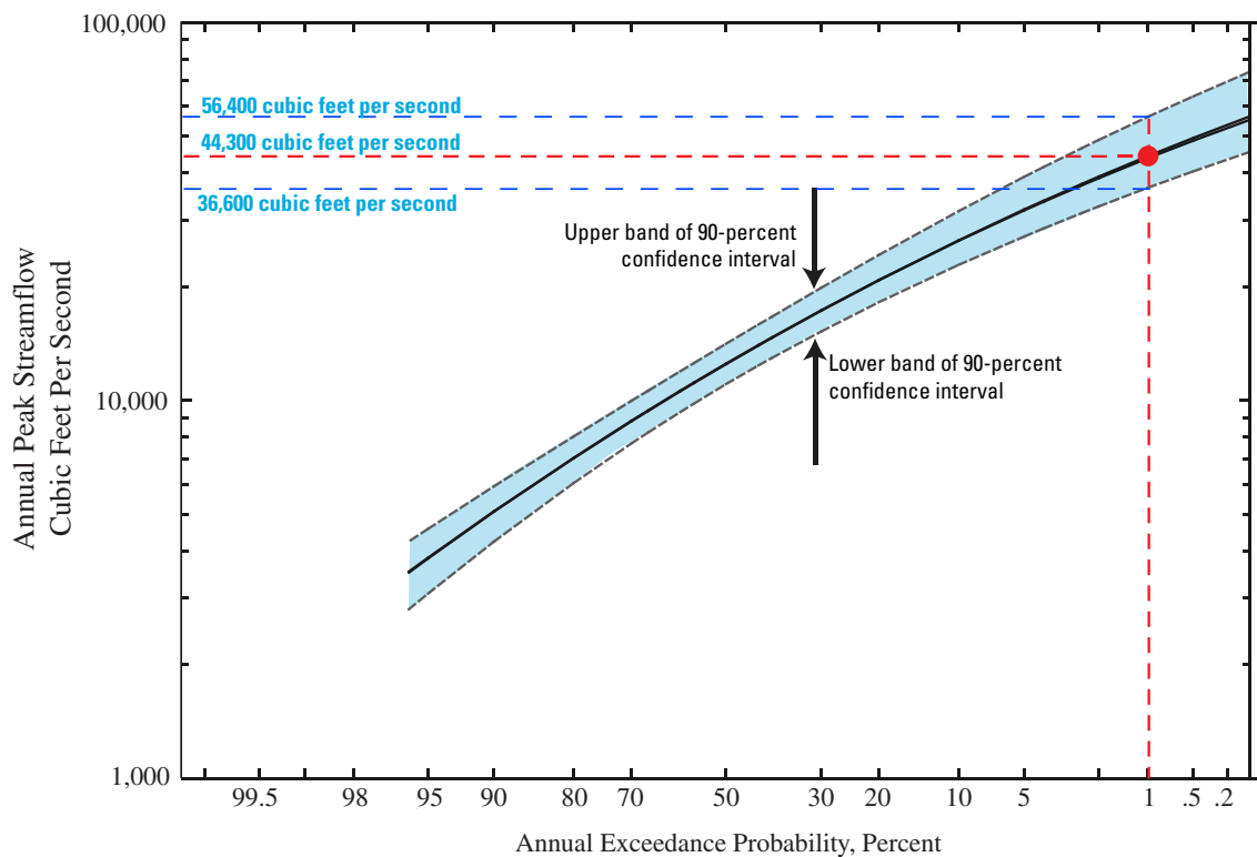
Solid line through data indicates fitted frequency curve; dashed lines indicate 90-percent confidence limits for the Big Piney River near Big Piney, MO.
