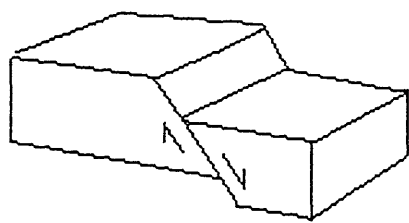
Normal fault
