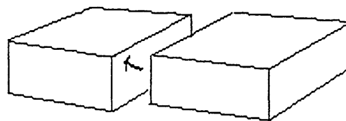
Oblique-slip fault
