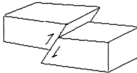
Reverse fault
