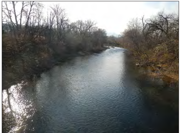
Site 7. Roanoke River above Bridge Street Bridge at Roanoke, Virginia, winter 2014. View from Bridge Street upstream.
