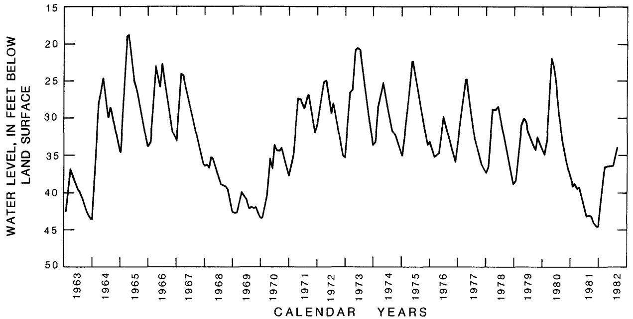
Figure 19A.— Monthly water levels in well 13L003 at Albany during 1963-82.
