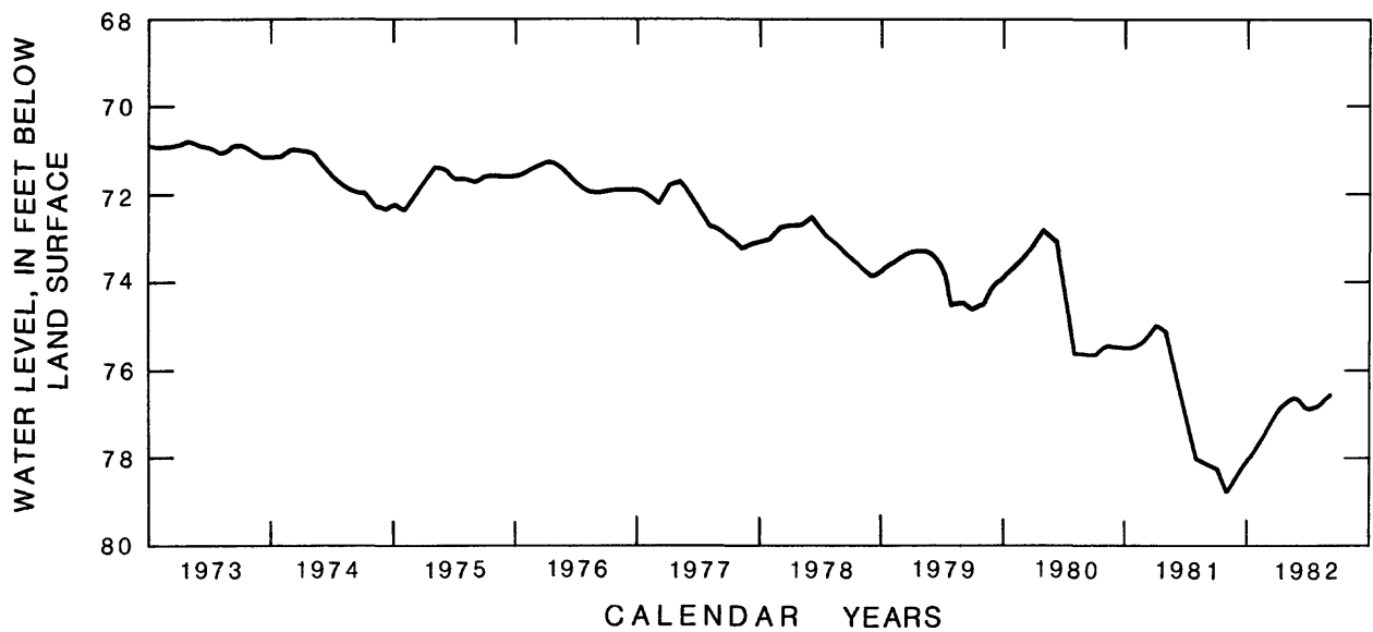
Figure 20A.— Monthly water levels in well 25Q1 at Uvalda School at Uvalda during 1973-82.
