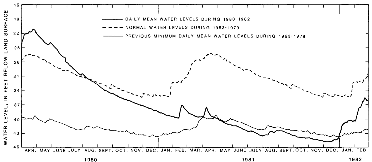
Figure 19B.— Daily mean water levels in well 13L003 at Albany, April 1980-February 1982.
