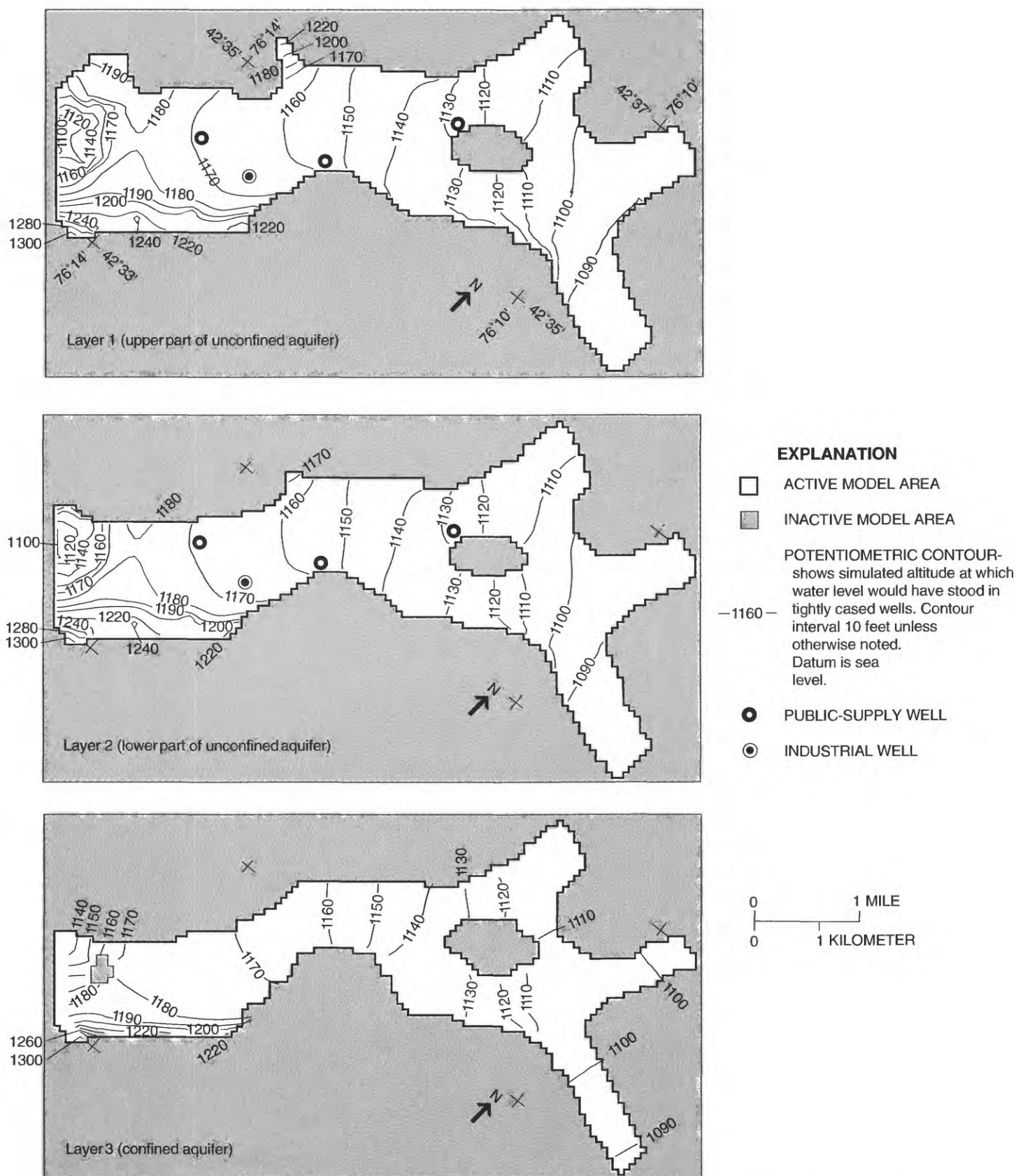
Figure 25B. Simulated head in model layers 1, 2, and 3 during steady-state average-recharge conditions in Cortland, N.Y. study area. (Locations and vertical positions of layers are shown in fig. 23.)
