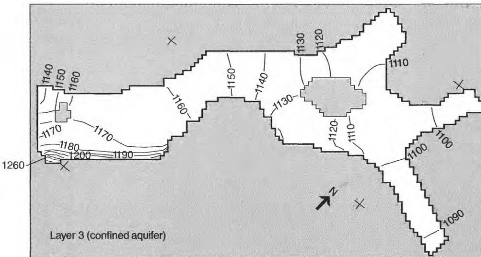
Figure 25C. Simulated head in model layers 1, 2, and 3 during steady-state low-recharge conditions in Cortland, N.Y. study area. (Locations and vertical positions of layers are shown in fig. 23.)
