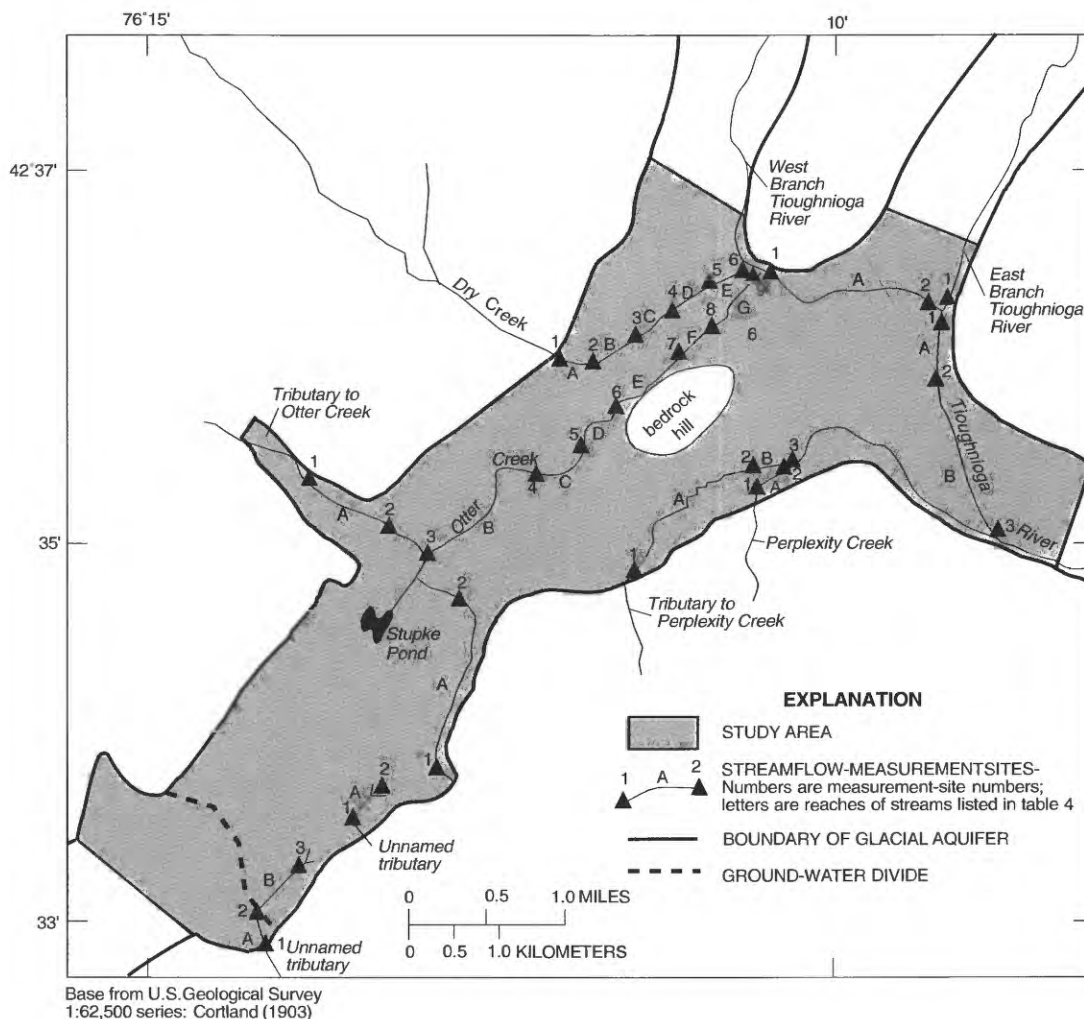
Figure 14. Location of streamflow-measurement sites in Cortland, N.Y., study area.
