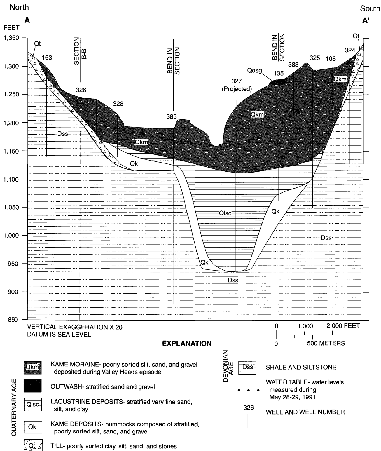
Figure 7A. Hydrogeologic section A-A'. (Line of section and well locations are shown in pl. 1.)
