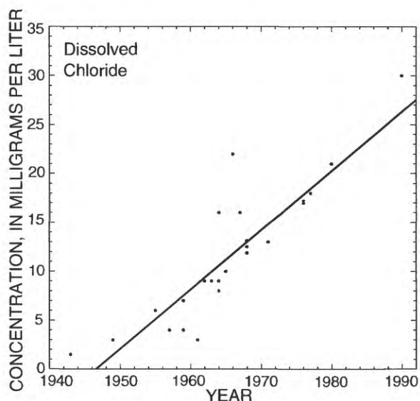
Figure 20. Dissolved chloride concentrations in water from wells at City of Cortland well field, 1943-76, 1980, and 1990. (Modified from Buller and others, 1978, fig. 20.)
