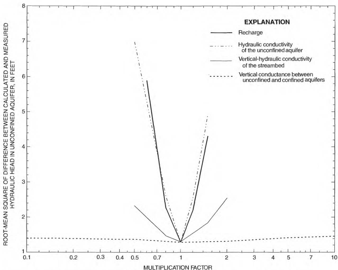
Figure 26. Results of sensitivity analyses for hydraulic head in unconfined aquifer in Cortland, N.Y. study area. (Root-mean squared calculated at 48 model cells containing observation wells.)
