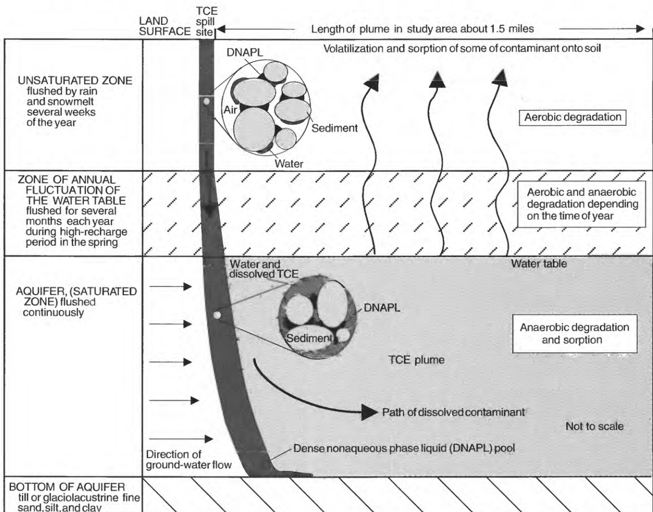
Figure 18. Physical, chemical, and biological processes that affect the fate and distribution of trichloroethylene (TCE) in and above the unconfined aquifer at Cortland, N.Y.
