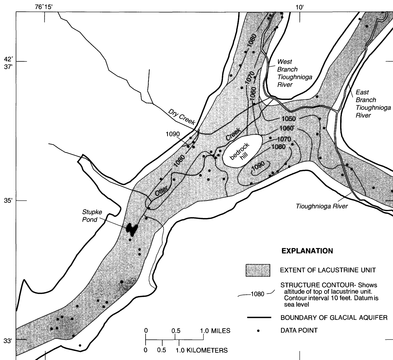
Figure 10. Upper surface altitude of lacustrine unit in Cortland, N.Y., study area.
