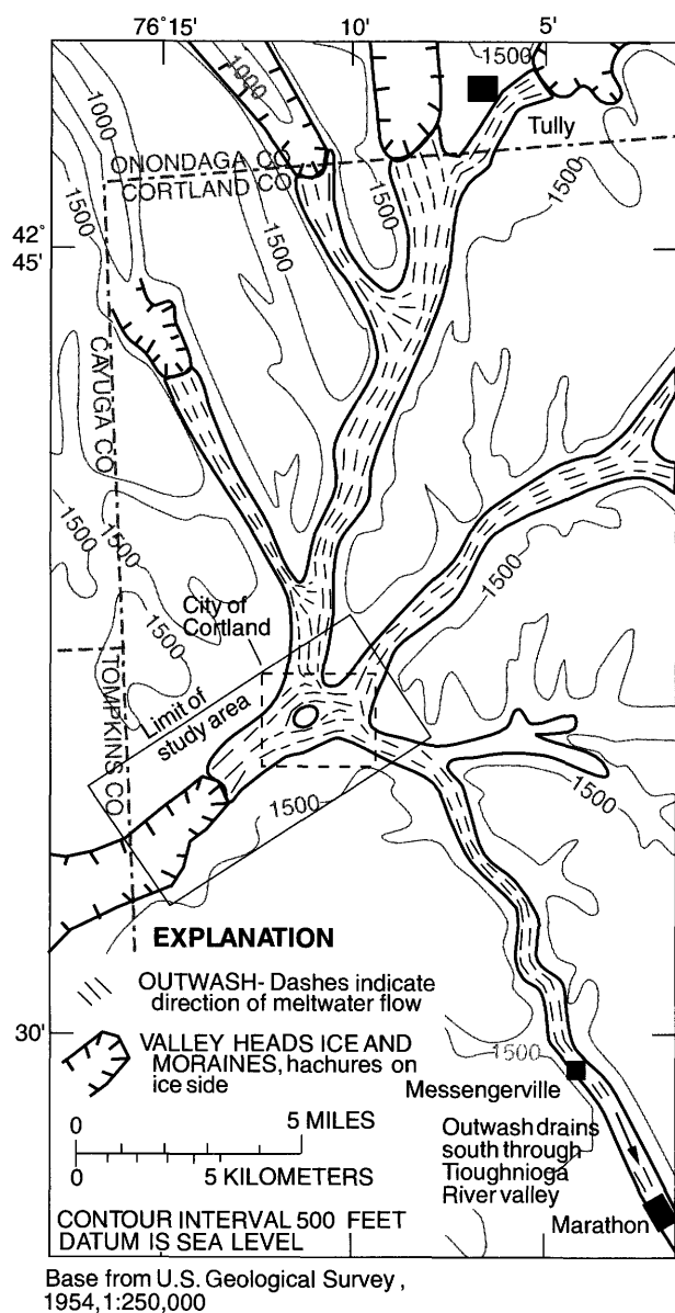
Figure 11. Positions of Valley Heads ice, and of outwash that was deposited in valleys of the Tioughnioga River basin. (Location is shown in fig. 9.)
