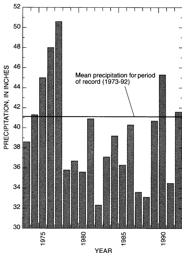
Figure 4. Annual precipitation at Cortland, N.Y., 1973-92. (Data from National Oceanic and Atmospheric Administration, 1992)
