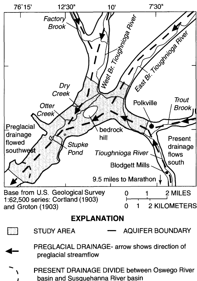
Figure 6. Preglacial drainage in Cortland, N.Y., study area.
