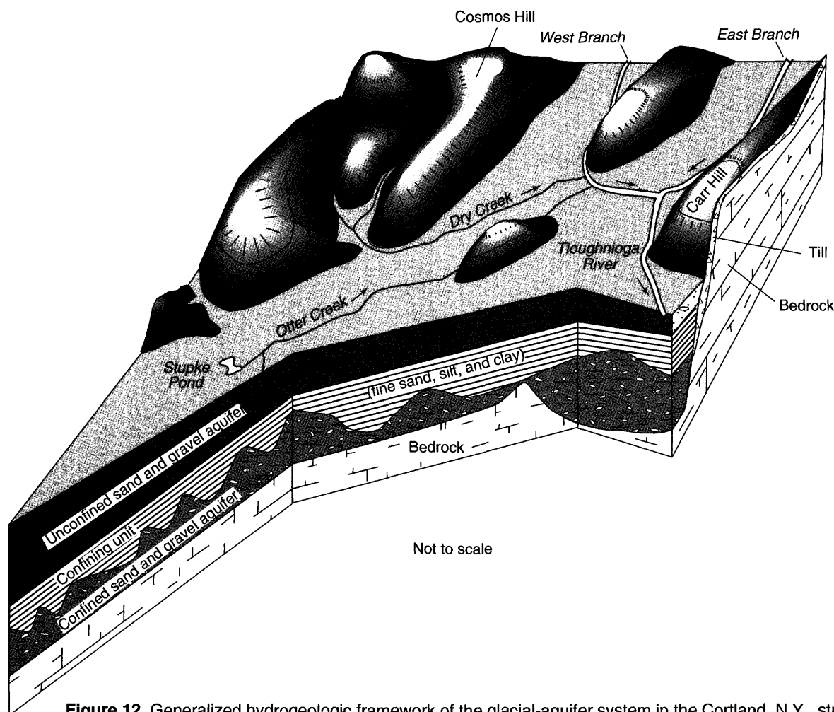
Figure 12. Generalized hydrogeologic framework of the glacial-aquifer system in the Cortland, N.Y., study area.
