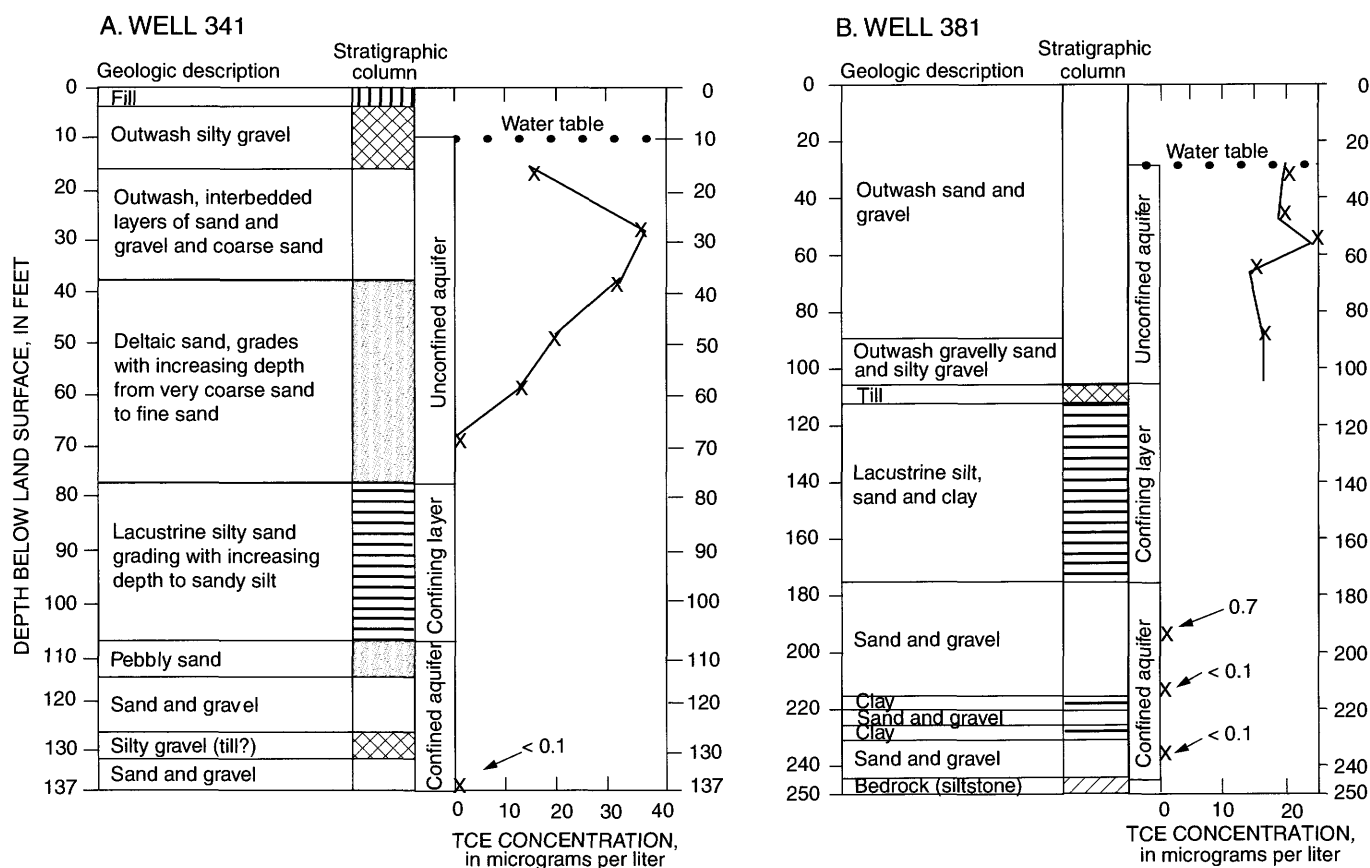
Figure 16. Vertical distribution of trichloroethylene (TCE) in ground water at two wells in Cortland, N.Y., study area: A. Well 341, 4,000 feet northeast of typewriter plant site, July 19, 1990. B. Well 381, 750 feet northeast of plant site, September 23-26, 1992. (Well locations shown on pl. 1.)
