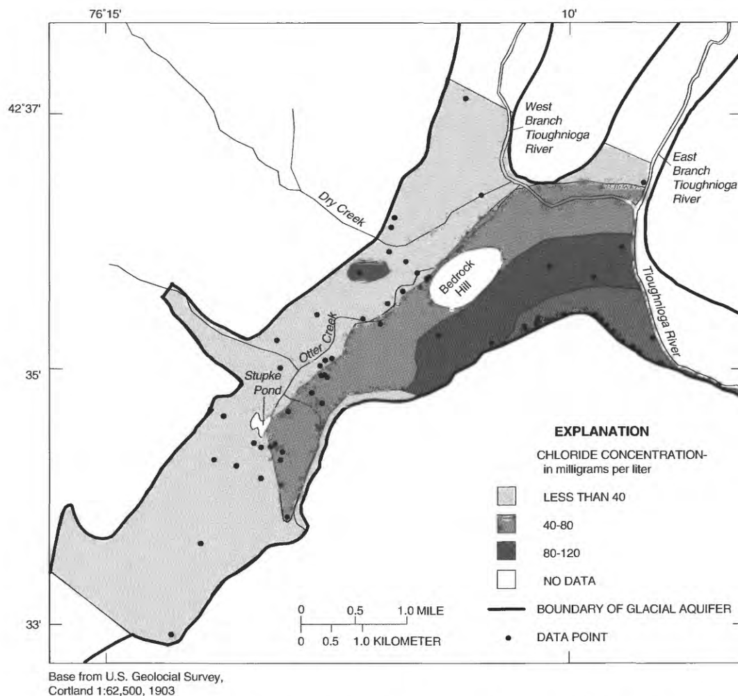
Figure 21. Distribution of chloride concentrations in the unconfined aquifer in Cortland study area, April 1990.
