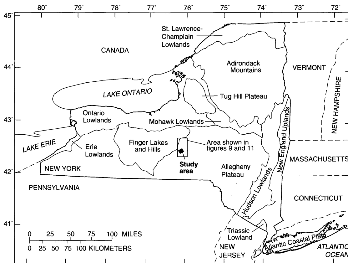
Figure 2. Physiographic features of New York. (Modified from Cressey, 1966, fig. 9, p. 26.)
