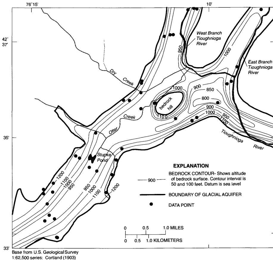
Figure 8. Bedrock-surface altitude in Cortland, N.Y., study area.
