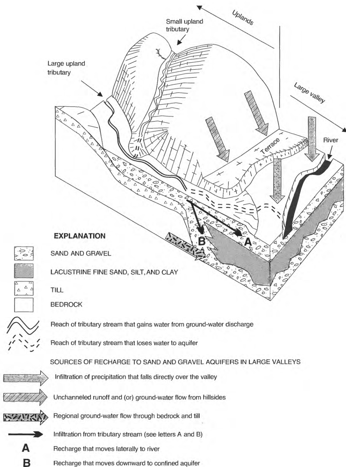
Figure 13. Sources of recharge to stratified drift in valleys in the glaciated Northeast. (Modified from Morrissey and others, 1987, fig. 1.)
