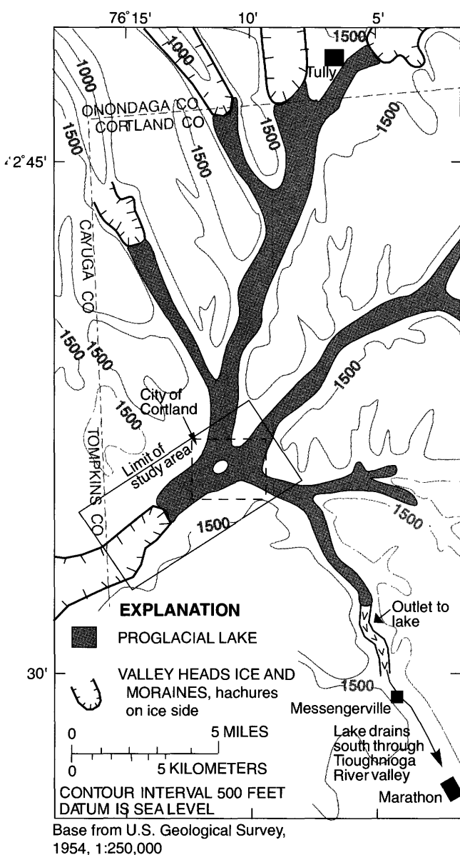
Figure 9. Location of Valley Heads ice and moraines that dammed drainage in valleys of the Tioughnioga River basin. (Location is shown in fig. 2.)
