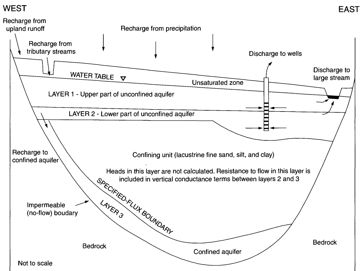
Figure 23. Conceptual model of ground-water flow in glacial-aquifer system in Cortland, N.Y., study area.
