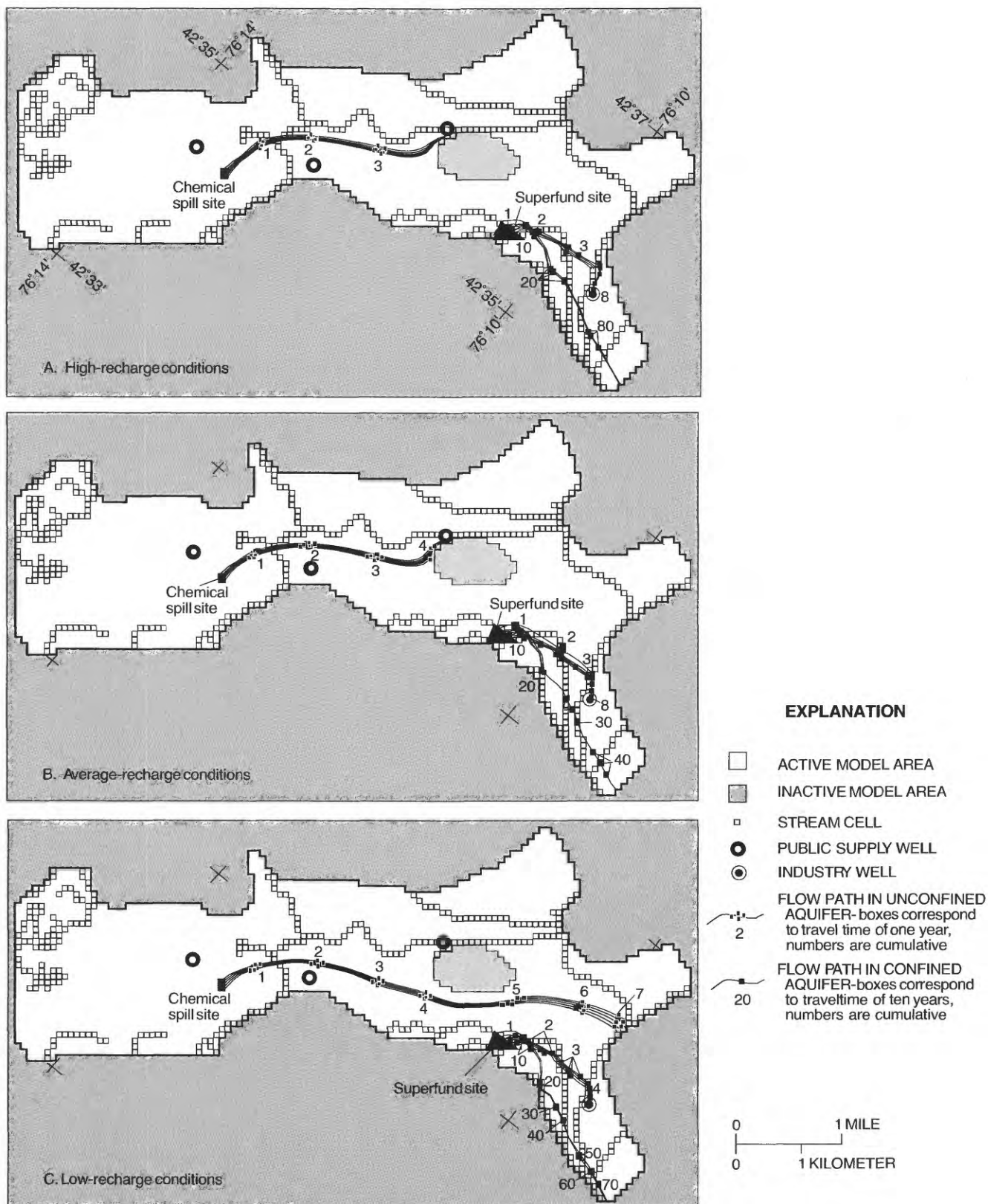
Figure 28. Flowpaths and traveltime of ground water moving from two contaminant sources in Cortland, N.Y. study area: A. Under high-recharge conditions. B. Under average-recharge conditions. C. Under low-recharge conditions. (Location is shown in fig.24.)
