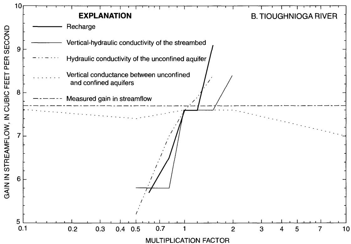
Figure 27. Results of sensitivity analyses for ground-water discharge to major streams during average-recharge conditions in the glacial-drift aquifer in the Cortland, N.Y. study area: A. Reach A of West Branch Tioughnioga River. B. Reaches A and B of Tioughnioga River. (Reach locations are shown in fig. 14.)
