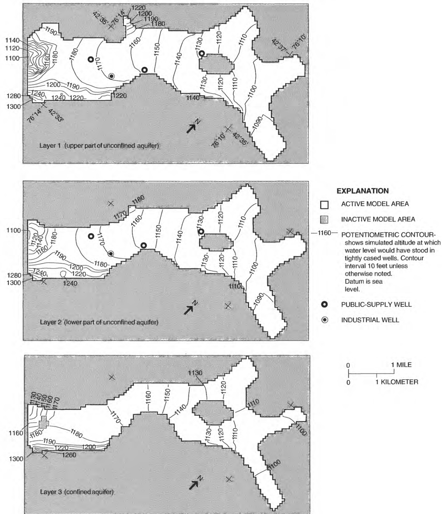
Figure 25A. Simulated head in model layers 1, 2, and 3 during steady-state high-recharge conditions in Cortland, N.Y. study area. (Locations and vertical positions of layers are shown in fig. 23.)
