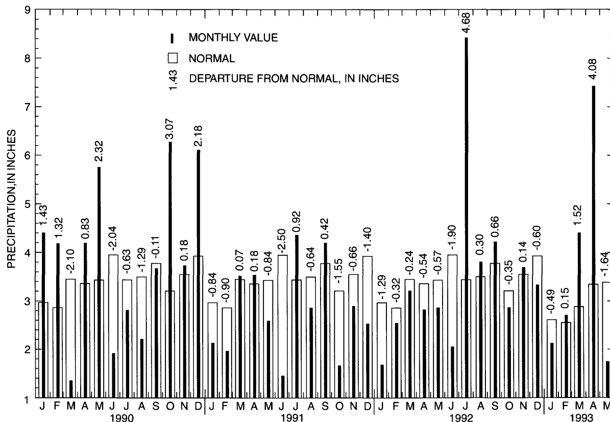
Figure 5. Monthly precipitation and departure from normal at Cortland, N.Y., January 1990 through May 1993. (Data from National Oceanic and Atmospheric Administration.)
