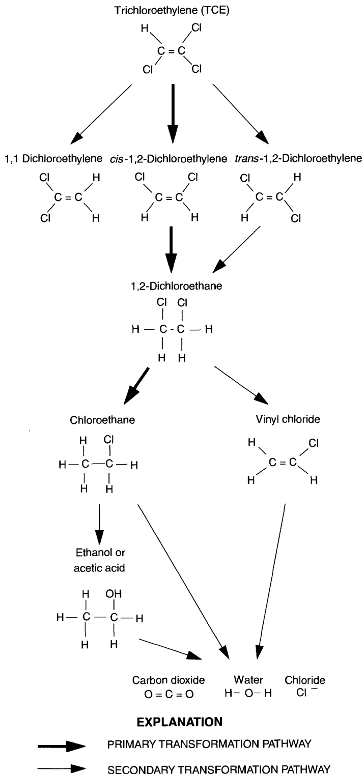
Figure 19. Transformation pathways of trichloroethylene under anaerobic conditions. (Modified from Davis and Olsen, 1990, fig. 1.)
