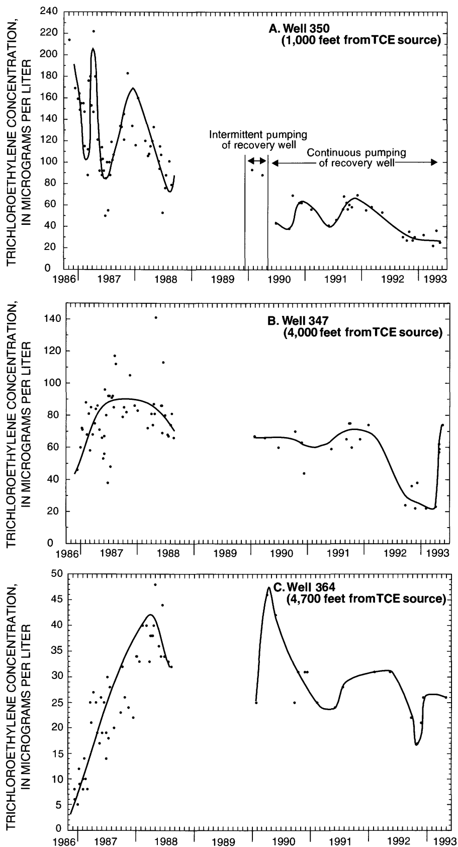
Figure 17. Trichloroethylene concentration at wells 350, 347, and 364 from November 1986 through May 1993. (Locations shown on pl. 1.)
