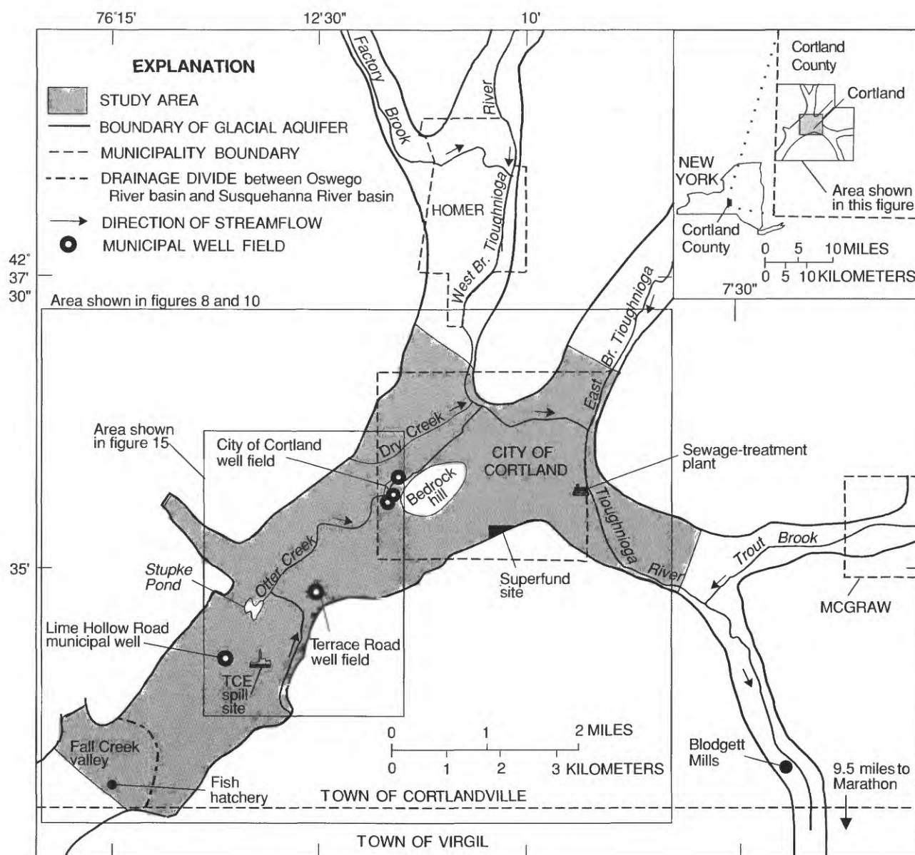
Figure 1. Location and principal geographic features of study area, Cortland County, N.Y.
