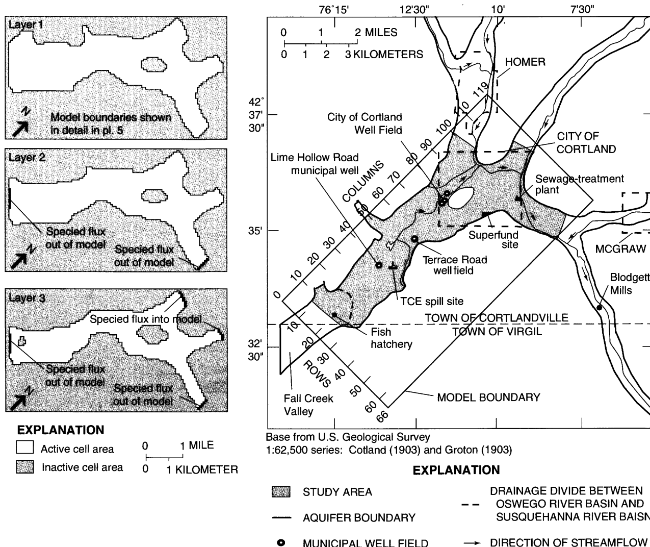
Figure 24. Locations of active and inactive grid boundaries in layers 1, 2, and 3 of the three-dimensional ground-water flow model of Cortland, N.Y. study area.
